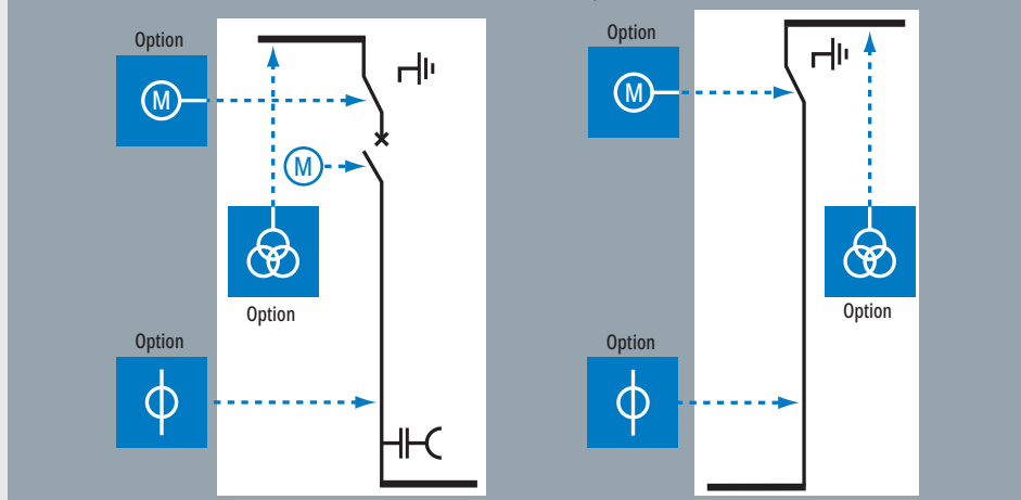
Sectionalizer and riser panel
