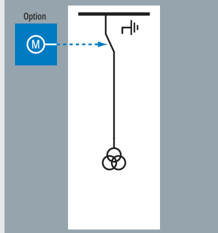
Busbar voltage measuring panel
